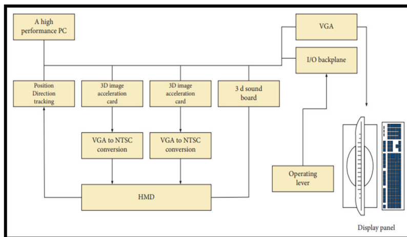
Figure 3: Diagram of the system architecture
