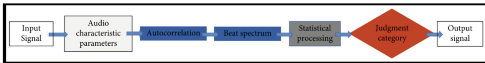
Figure 4: Algorithm flow
